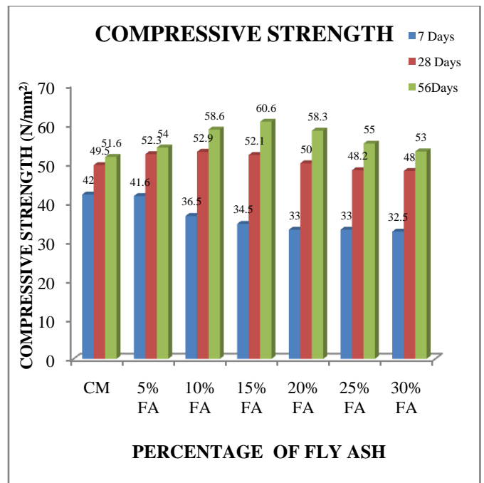
Fig 5: 7, 28, 56 Days Compressive Strength of fly ash mix
