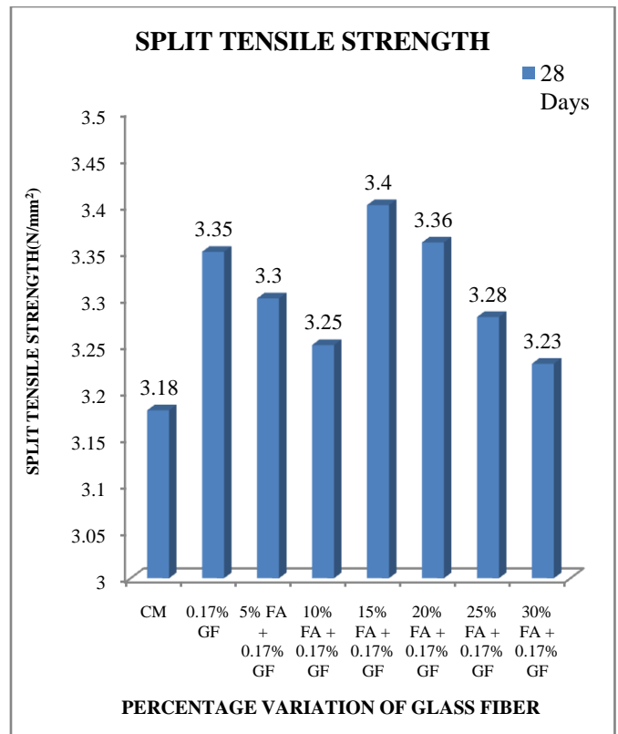
Fig 8: 28 Days Split Tensile Strength of FA+GF mix
