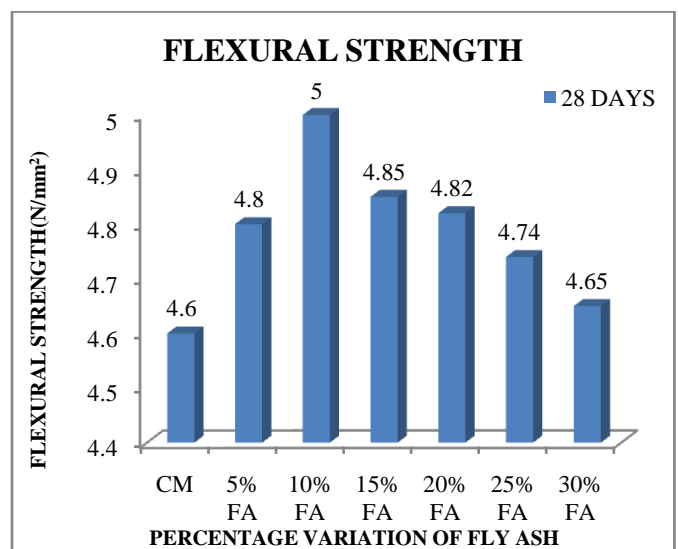
Fig 9: 28 Days Flexural Strength of FA mix
