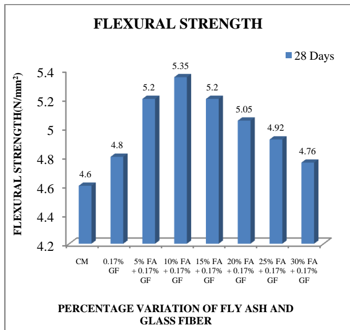
Fig 10: 28 Days Flexural Strength of GF+FA mix
