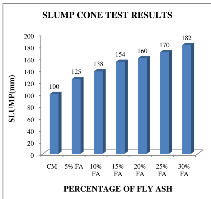
Fig. 11: Workability of fly ash concrete mix.
