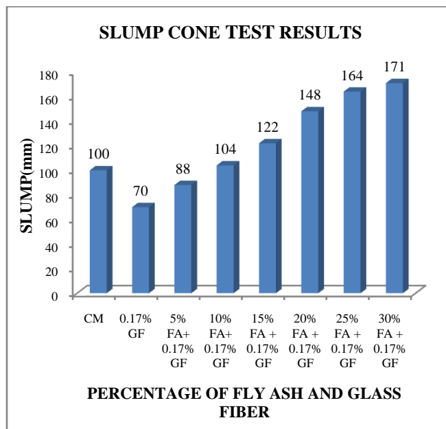
Fig 12: Workability of fly ash and glass fiber concrete mix.
