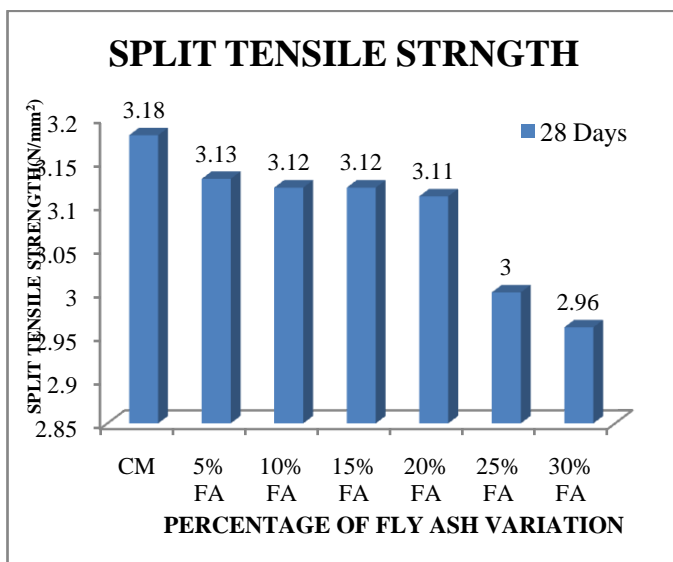
Fig 7: 28 Days Split Tensile Strength of FA mix
